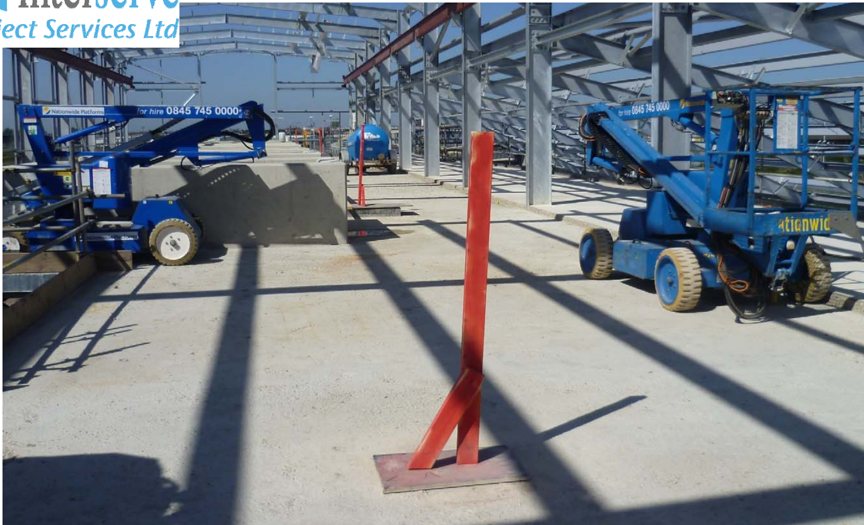
Safe, simple and effective protection over openings in floors: easily seen and thus easily avoided by MEWP operators
